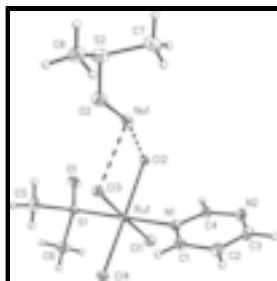
Fig. 1. A view of the title compound, with displacement ellipsoids shown at the 50% probability level.
